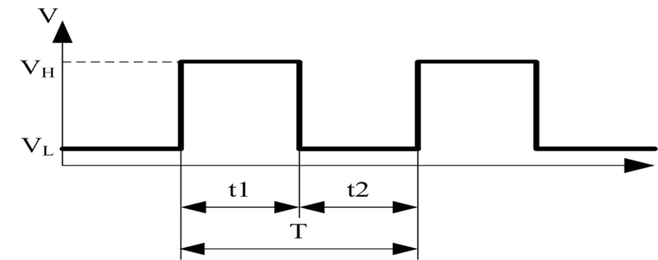
★PWM INPUT WAVEFORM
