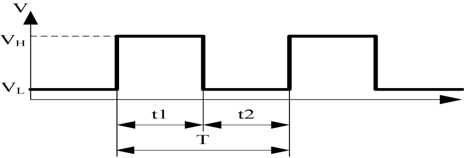
★PWM INPUT WAVEFORM
